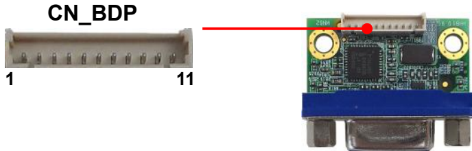
CN_BDP : DP to VGA 11-pin connector
