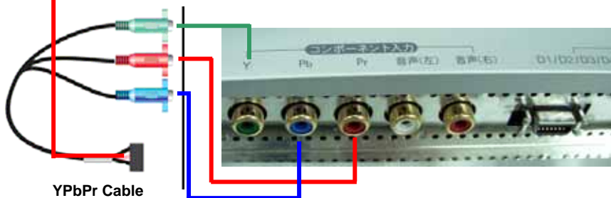
YPbPr Cable (Optional cable)
