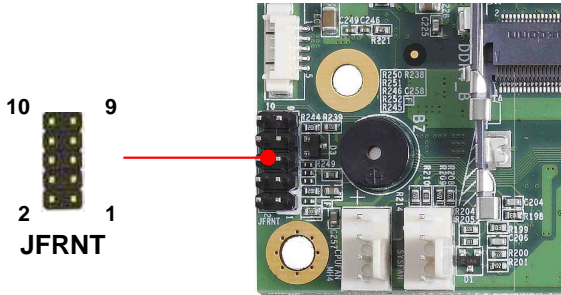
JFRNT: Front panel switch and indicator 14-pin header (Pitch 2.54mm)
