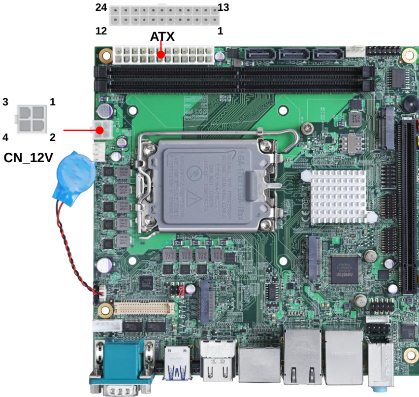
CN_12V: ATX12V 4-pin connector
