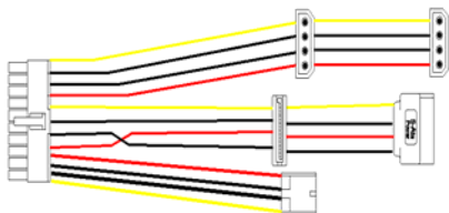
ATX Power Output Cable x 1 (OALATX-P3S2)
