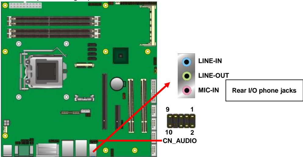
Connector: CN_AUDIO Type: 10-pin (2 x 5) header
