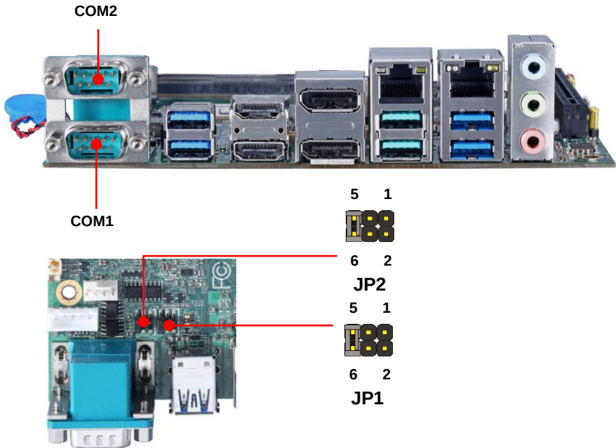
COM1: RS232/422/485 DB9 connector
